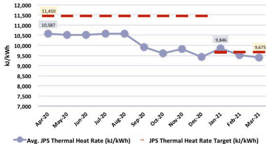
FIGURE 3: JPS'S MONTHLY HEAT RATE PERFORMANCE
